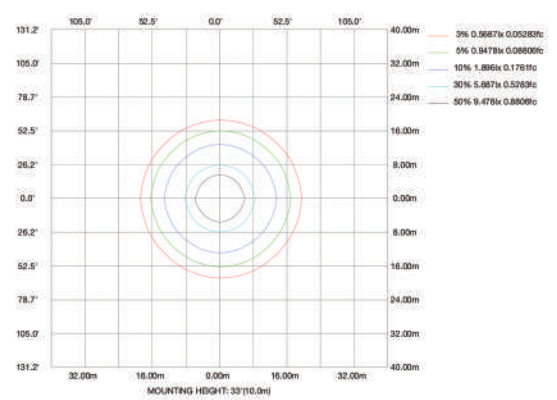
ISOLUX DIAGRAM
